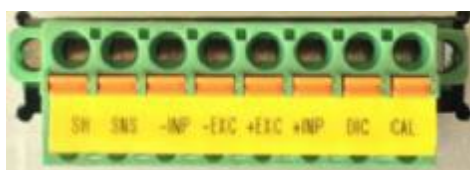
Phoenix Connector-8 pins
